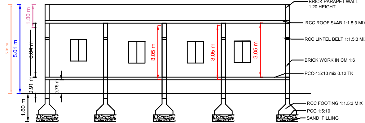
SECTION "AB"
