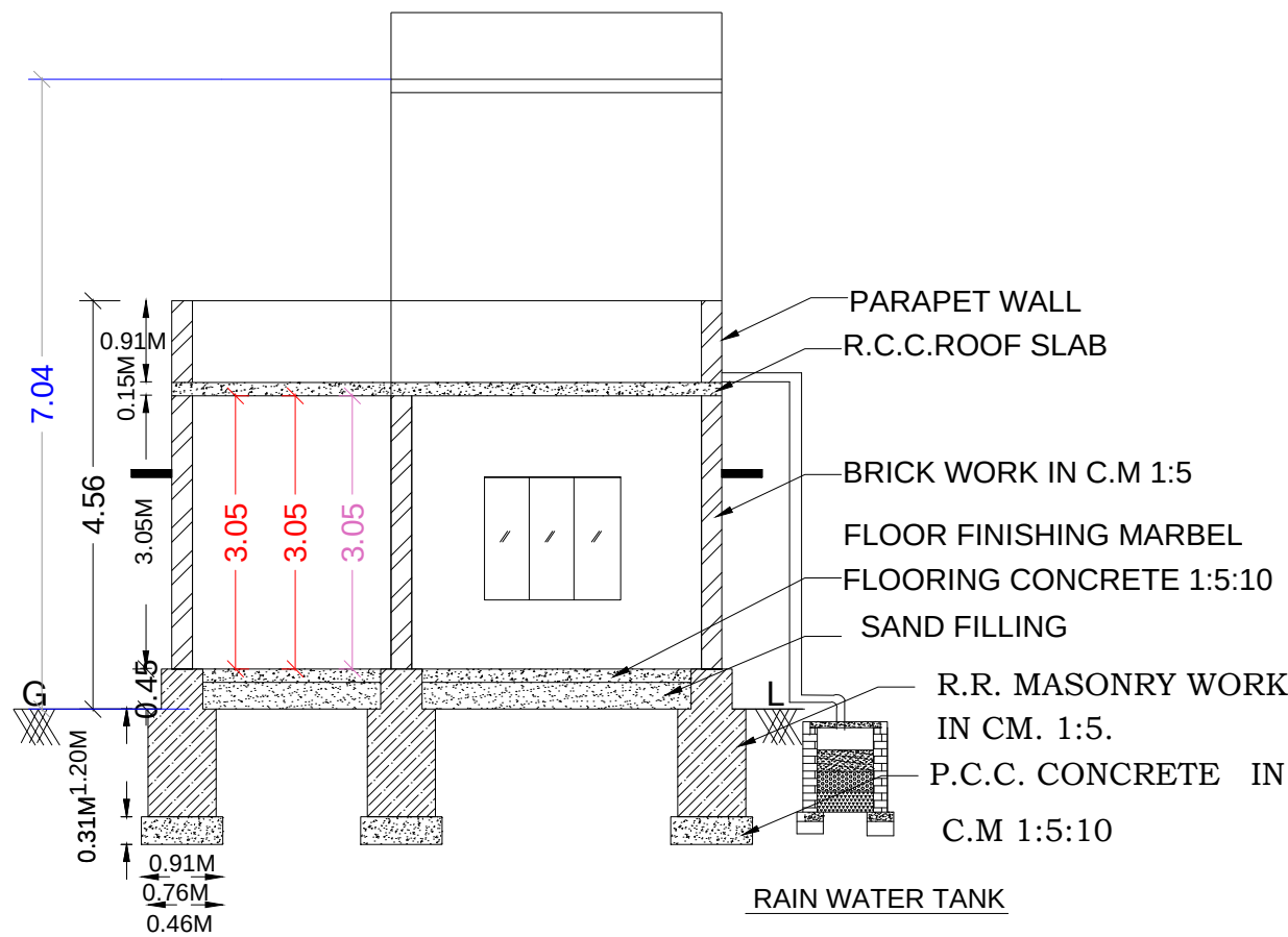
SECTION - XX
