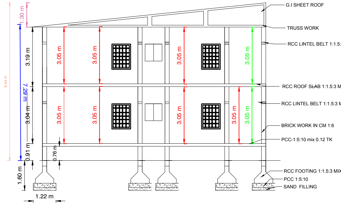
SECTION "AB"
