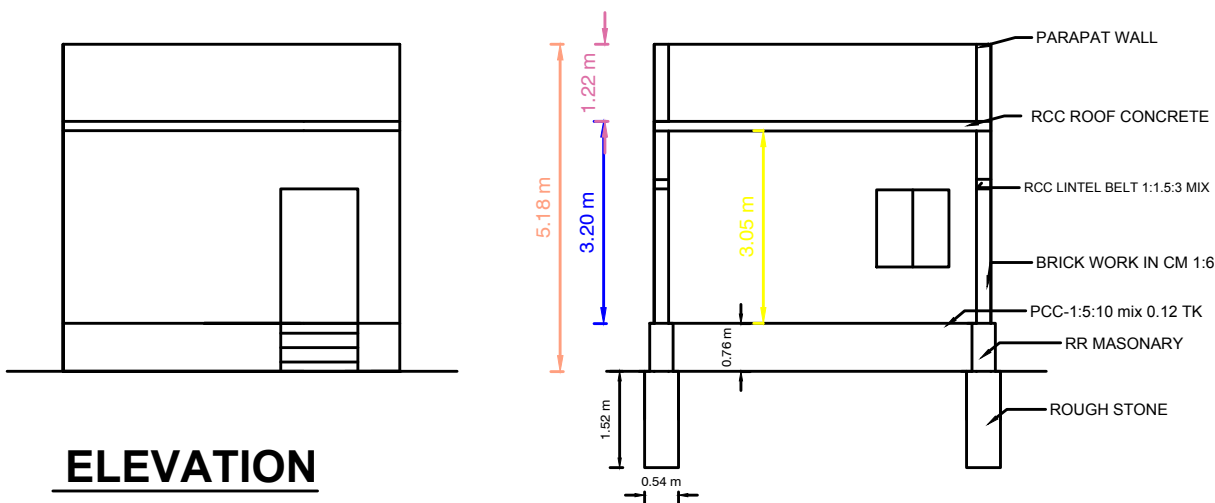
SECTION"AB"
