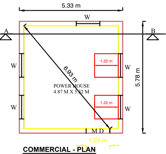
COMMERCIAL - PLAN
