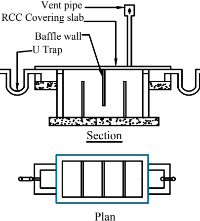
SECTION"AB"
