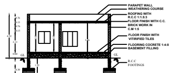
SECTION ON "S S"
