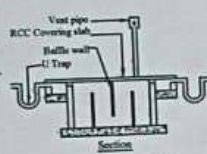
SECTION " AB "
