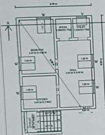
GROUND FLOOR PLAN : 707.85 SQ FT
