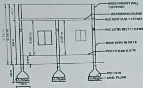
SECTION " AB "
