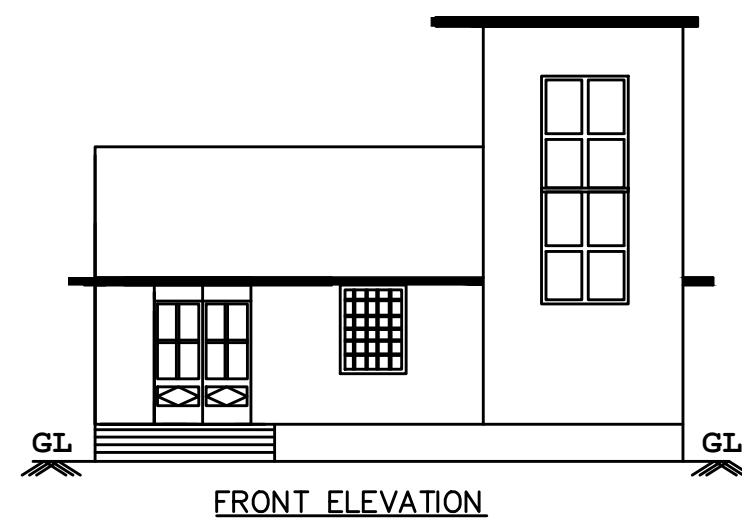
FRONT ELEVATION
