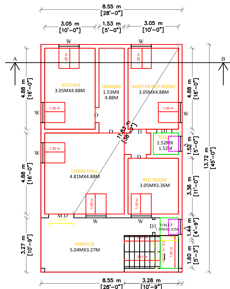
GROUND FLOOR PLAN ING TO
