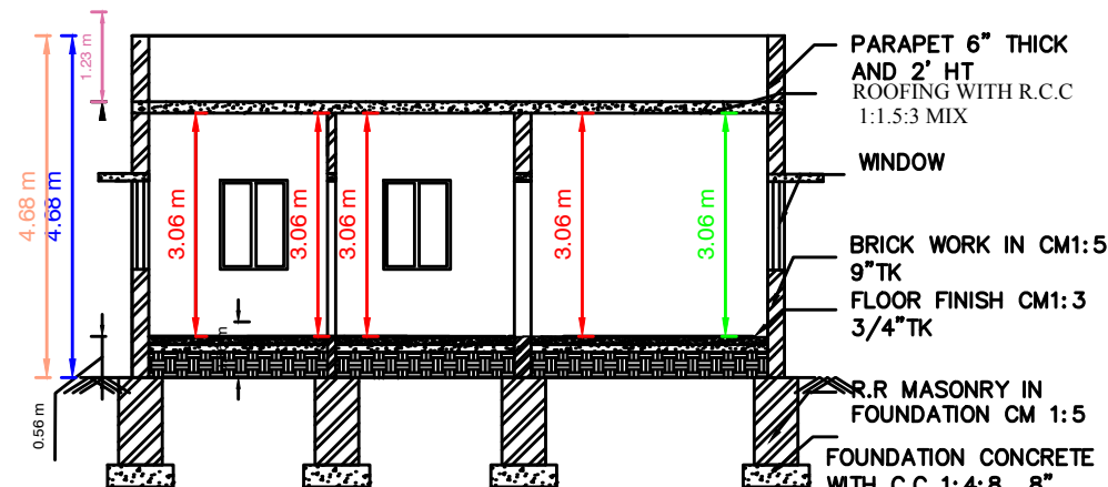
SECTIONAL VIEW A—A'
