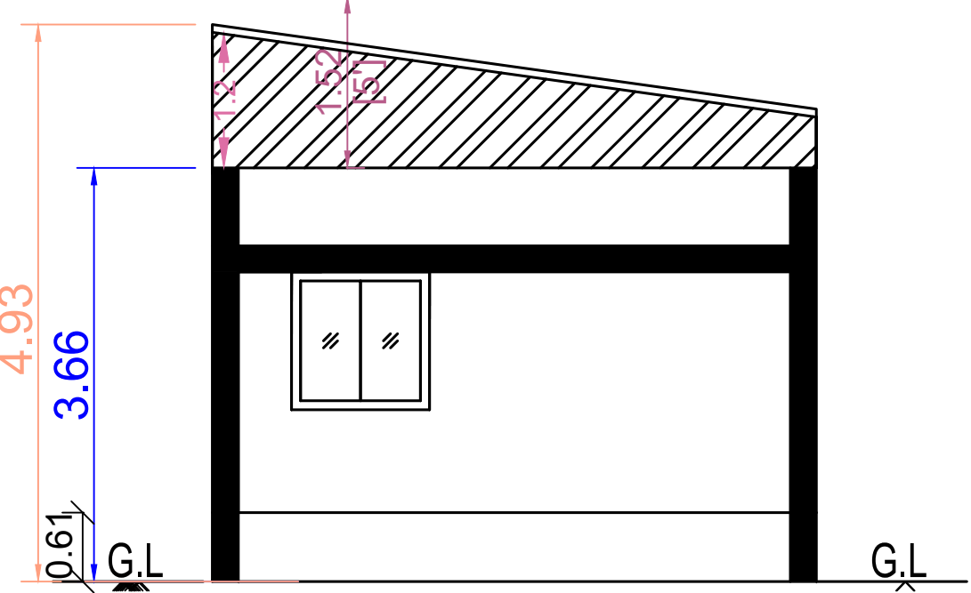
ELEVATION (SOUTH SIDE VIEW)
