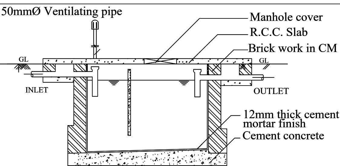
Longitudinal Section (SEPTIC TANK)
