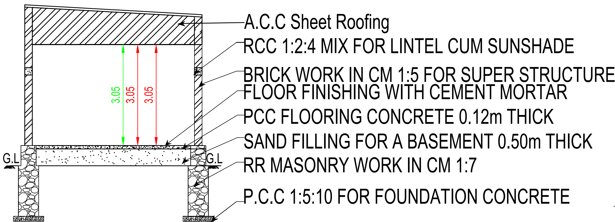
SECTION-"AA"
