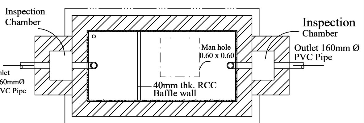
f Septic tank
