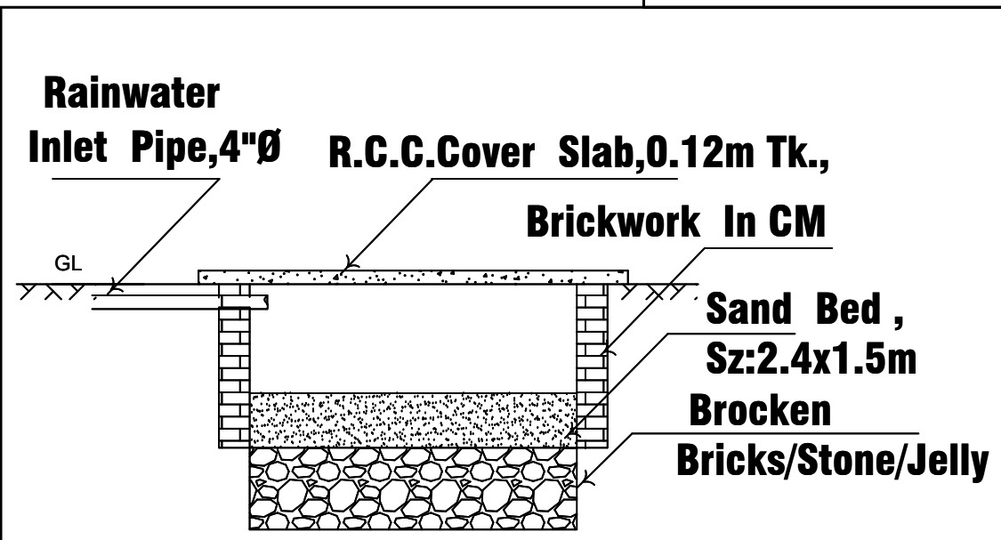
SECTION ON "MN"
