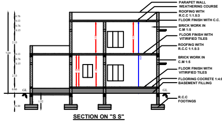
SECTION ON "S S"
