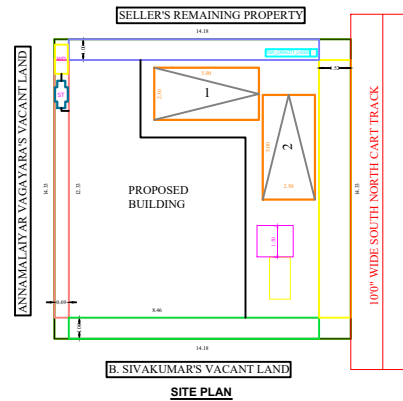
SITE PLAN
