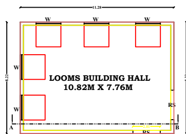
LOOMS BUILDING - PLAN
