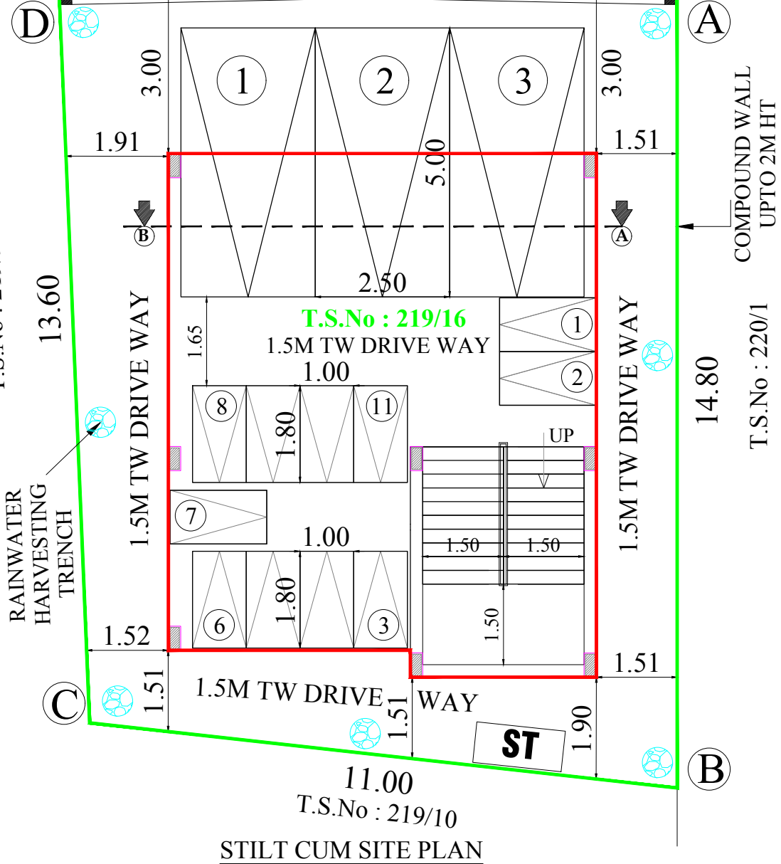
STILT CUM SITE PLAN
