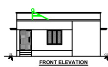
FRONT ELEVATION
