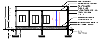
SECTION ON "S S"
