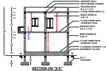
SECTION ON "S S"
