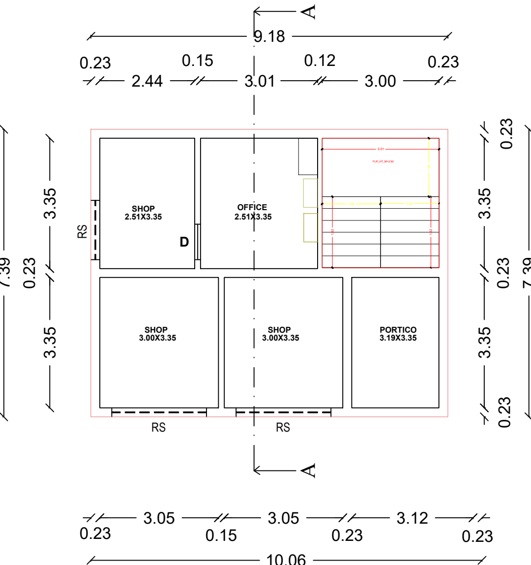
ALREADY APPROVED COMMERCIAL BUILDING GROUND FLOOR PLAN
