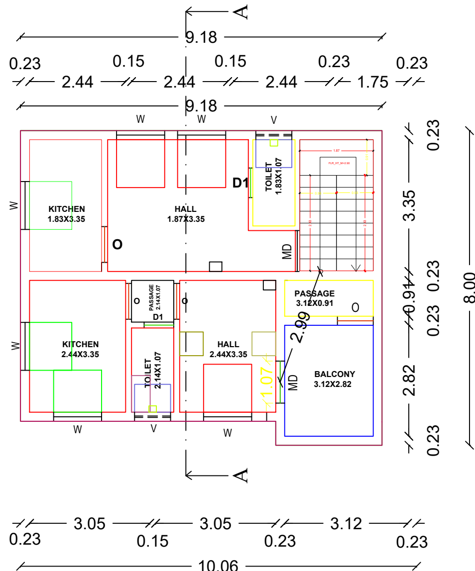
ALREADY APPROVED RESIDENTIAL BUILDING FIRST FLOOR PLAN
