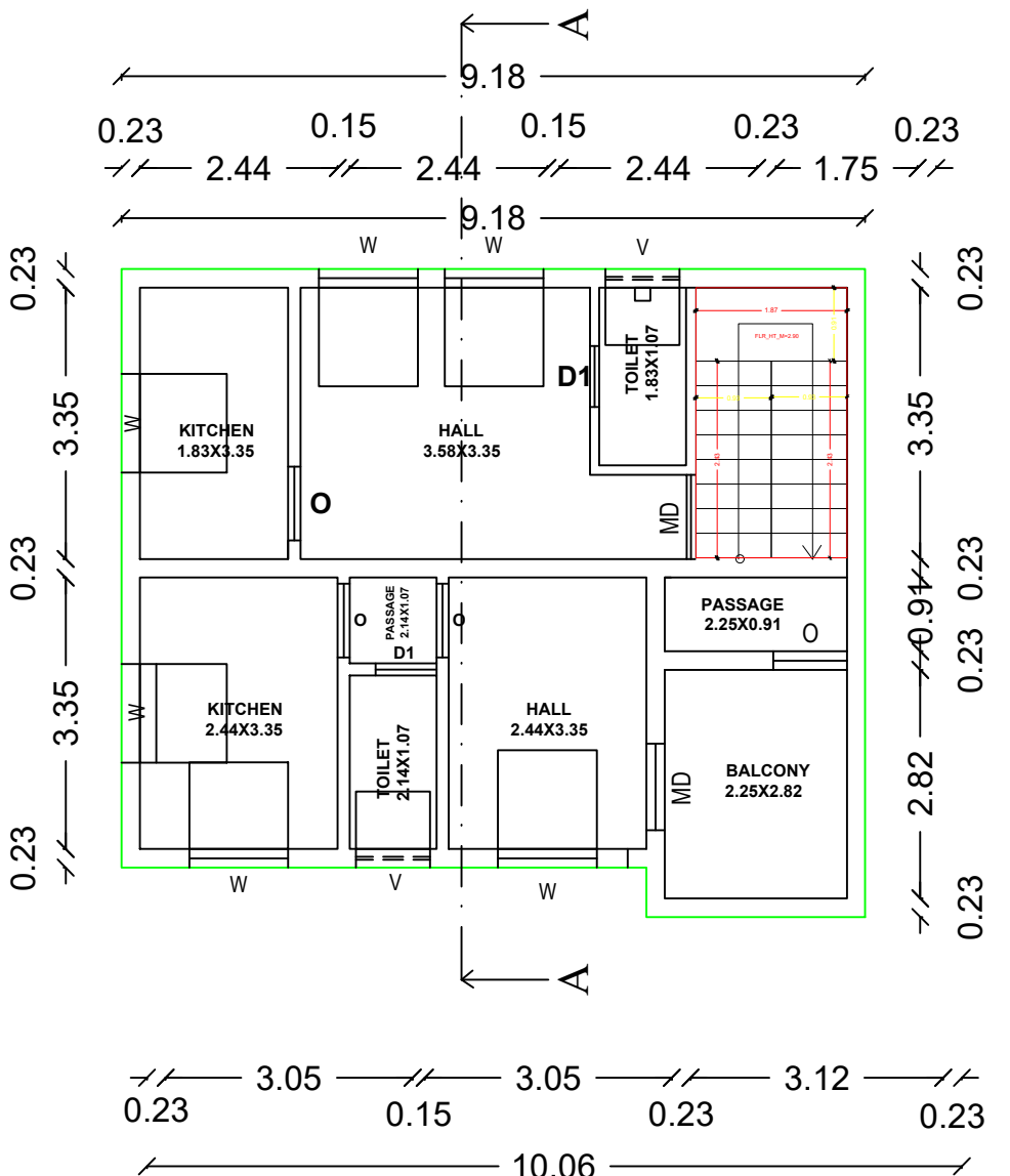
ALREADY APPROVED RESIDENTIAL BUILDING FIRST FLOOR PLAN
