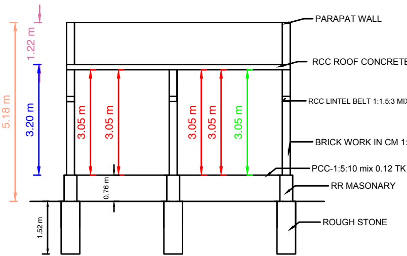
SECTION"AB"
