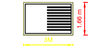
WATER TANK _2000 LITER
