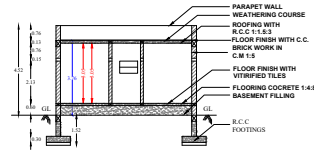
SECTION ON "S S"
