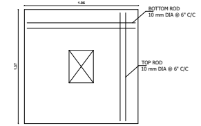
FOOTING PLAN
