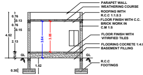
SECTION ON "S S"
