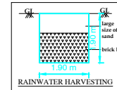
RAINWATER HARVESTING RAIN TANK CAPACITY=2000LITER
