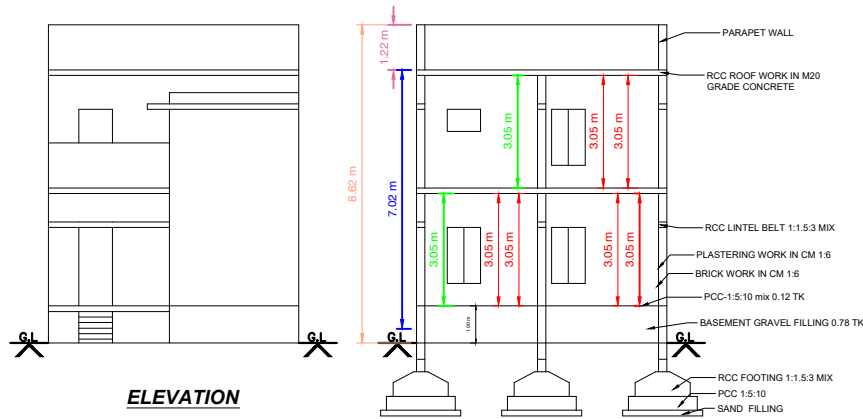
SECTION"AB"
