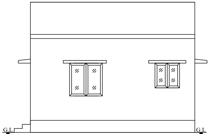
BLOCK-2 ELEVATION
