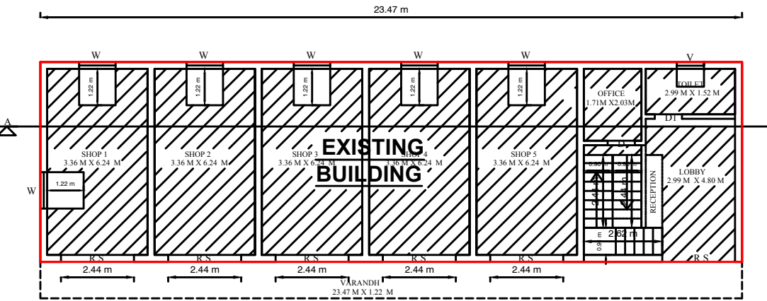
GROUND FLOOR ( EXISTING )
