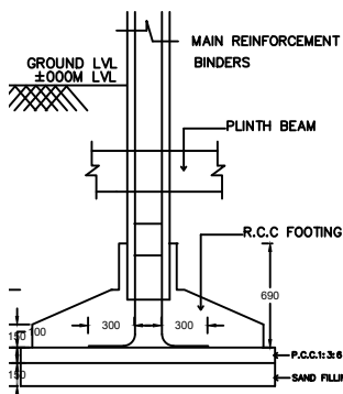
TYPICAL SECTION OF R.C.C. COLUMN FOUNDATION SCALE : 1" = 2'-0"
