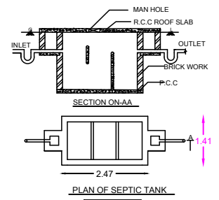
PLAN OF SEPTIC TANK NOT TO SCALE
