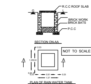
PLAN OF RAIN WATER TANK NOT TO SCALE
