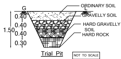
Trial Pit NOT TO SCALE
