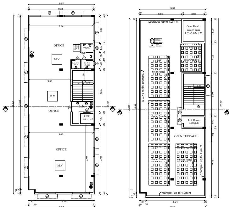
First & Second floor plan
