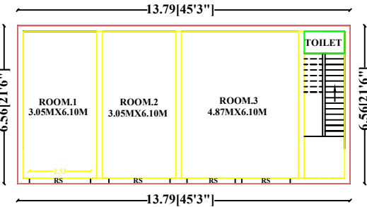
GROUND FLOOR COMMERCIAL - PLAN
