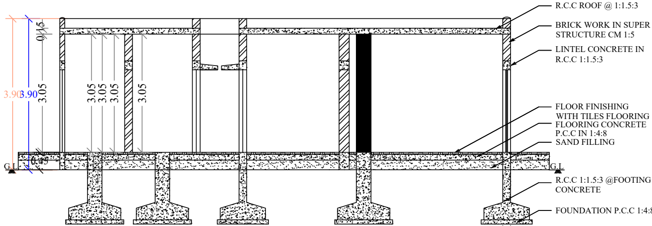
SECTION-AB
