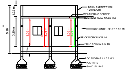
SECTION " AB "
