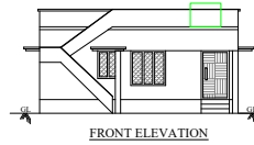
FRONT ELEVATION
