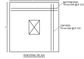
FOOTING PLAN
