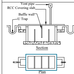
RAINWATER HARVESTING RWH TANK CAPACITY=2000LITER
