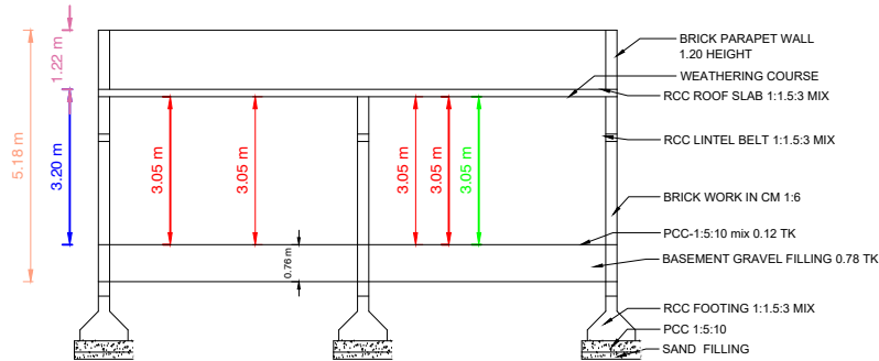
SECTION"AB"
