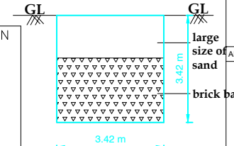
RAINWATER HARVESTING RWH TANK CAPACITY=2000LITER
