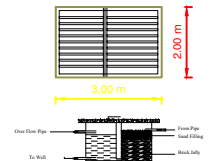
WATER TANK _2000 LITER
