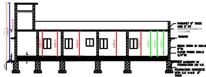
SECTIONAL VIEW A-A'
