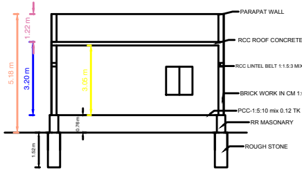
SECTION"AB"
