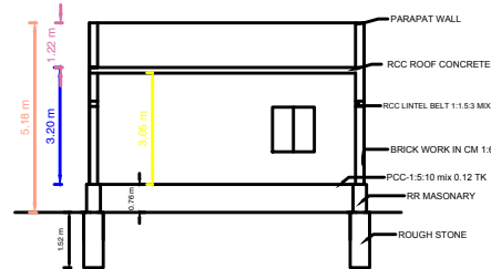
SECTION"AB"
