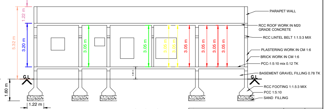
SECTION"AB"
