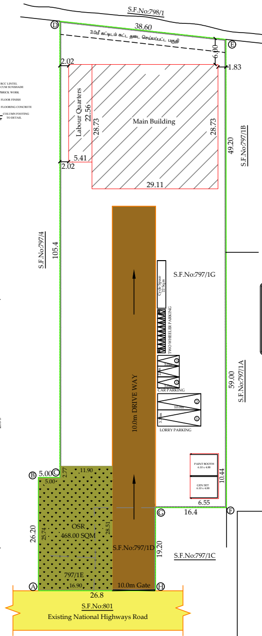
SITE PLAN
