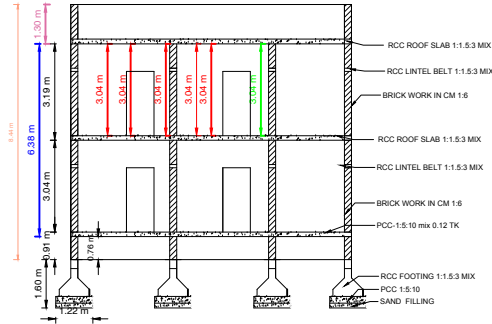
SECTION "AB"
