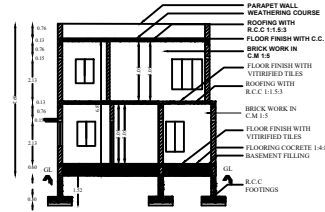
SECTION ON "S S"
