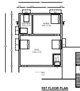
RST FLOOR PLAN
