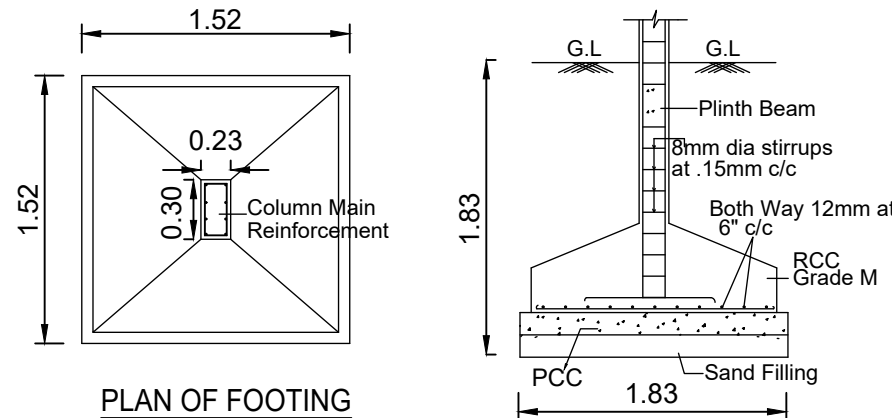
FOUNDATION DETAILS
