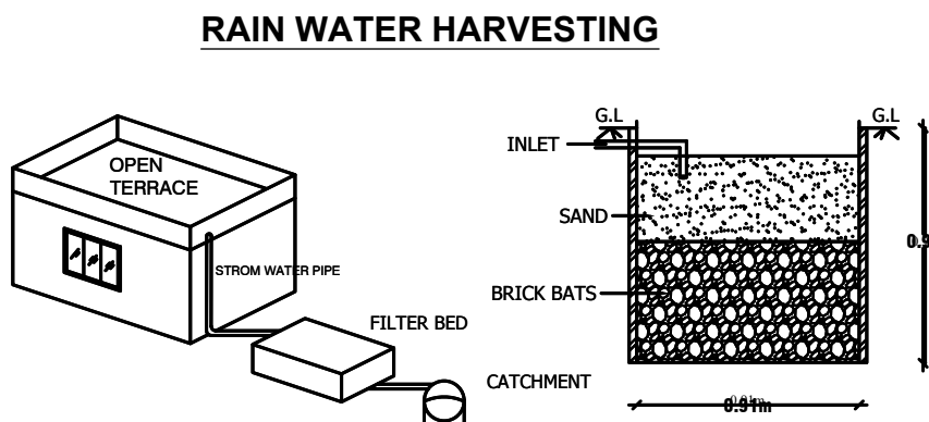
RAIN WATER COLLECTION PIT DETAILS SCALE - 1:100
