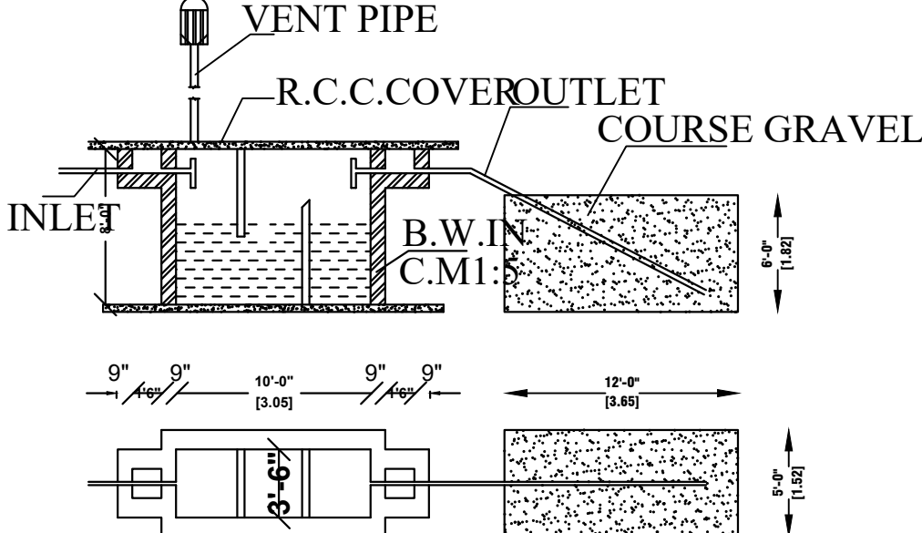
SEPTIC TANK & D-TRENCH DETAILS (NOT TO SCALE)
