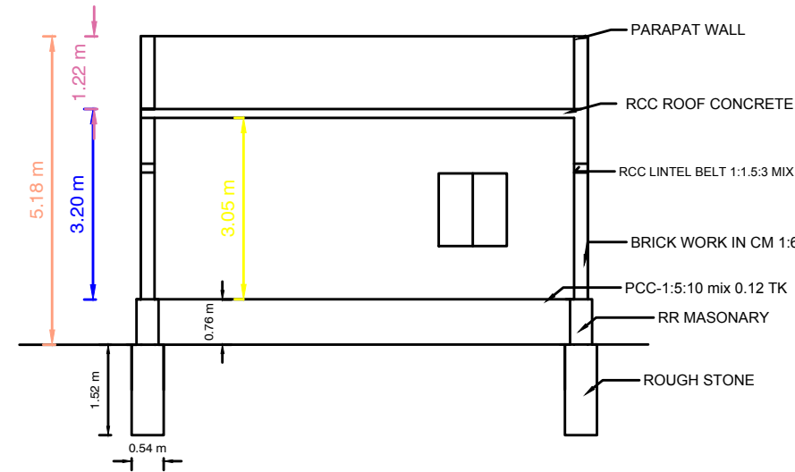
SECTION"AB"
