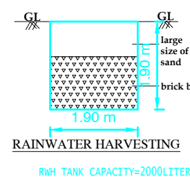
RWH TANK CAPACITY=2000LITER
