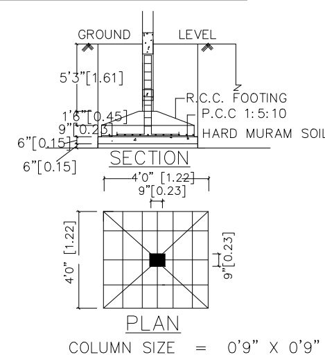
COLUMN SIZE
