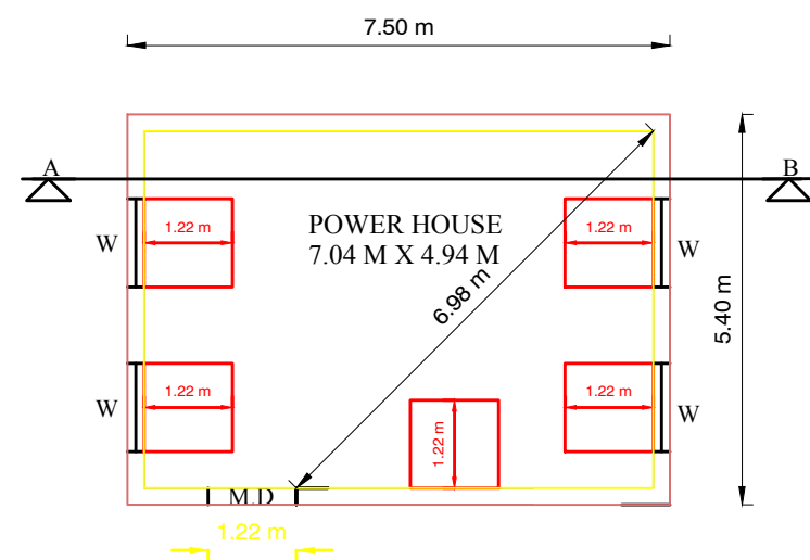
COMMERCIAL - PLAN
