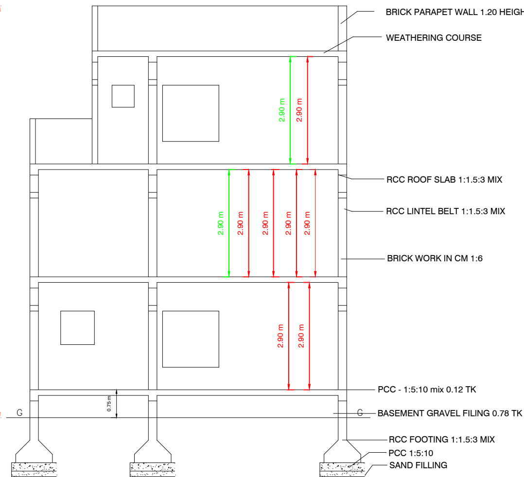
SECTION"AB"
