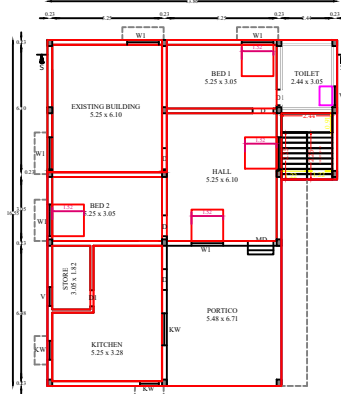
EXISTING AND PROPOSED
