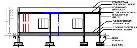
SECTION ON "S S"
