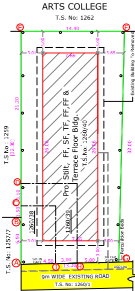
SITE PLAN
