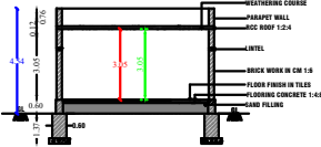
SECTION ON "S-S"
