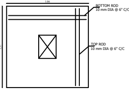
FOOTING PLAN
