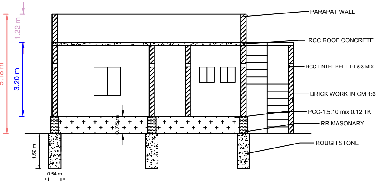
SECTION " AB "
