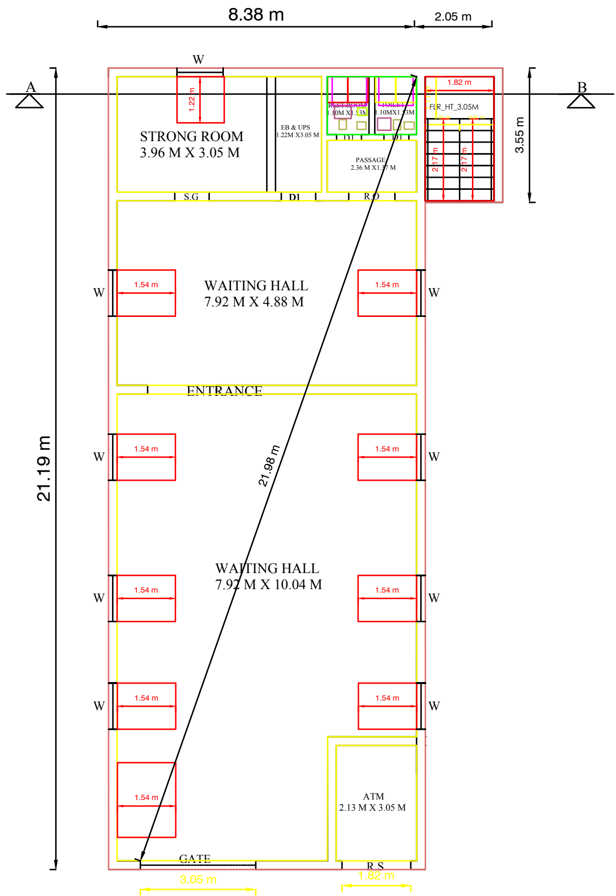
COMMERCIAL - PLAN
