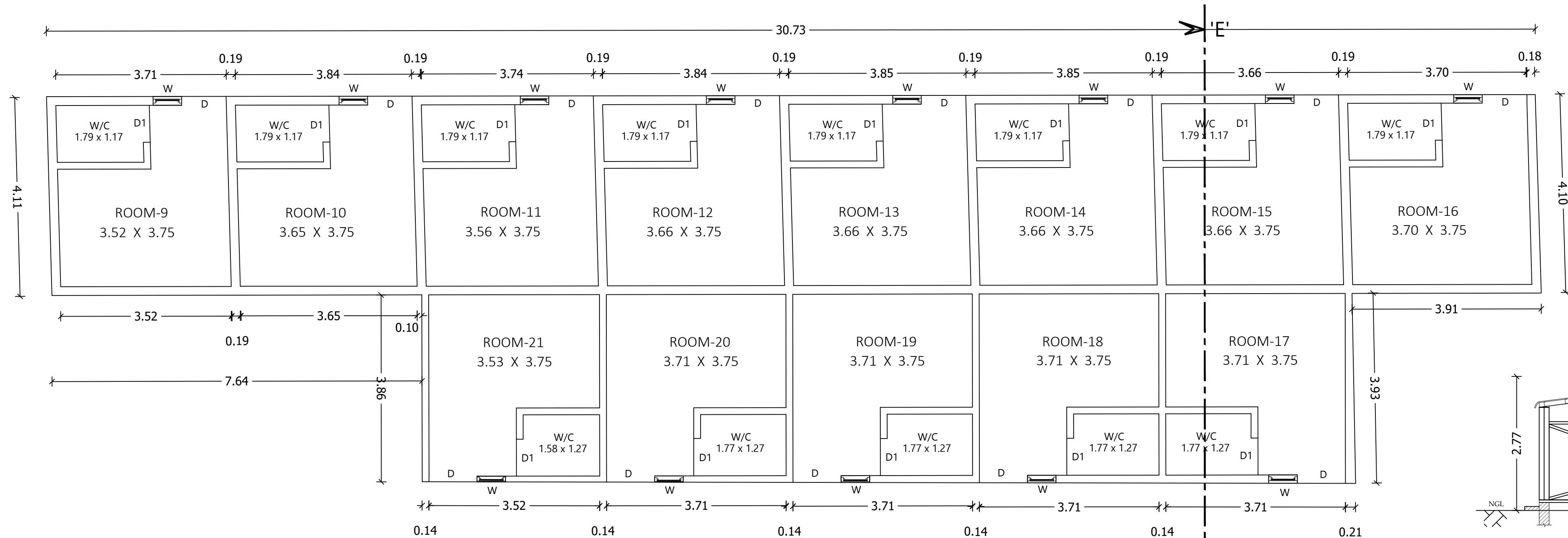
PLAN
