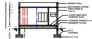
SECTION ON "S S"
