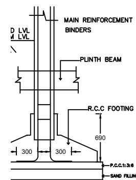
TYPICAL SECTION OF R.C.C. COLUMN FOUNDATION
