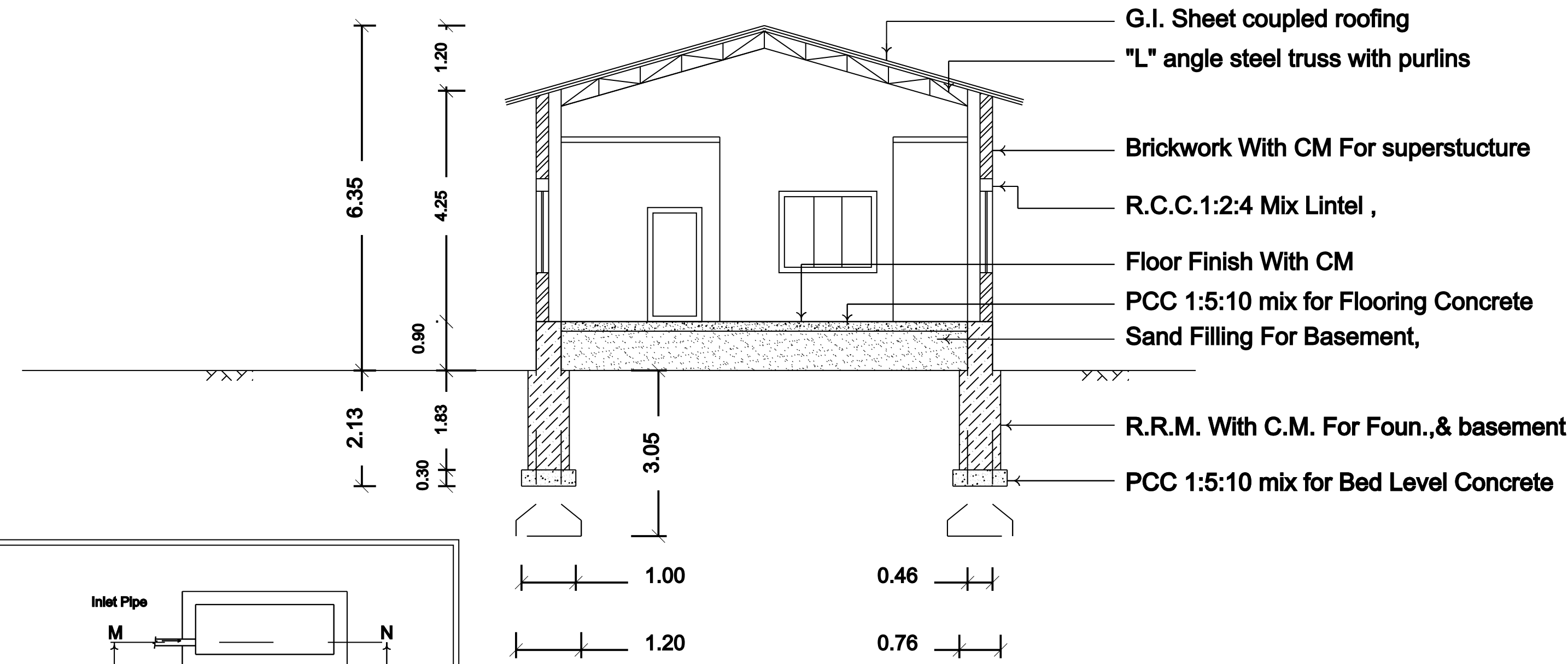
SECTION ON "XY"
