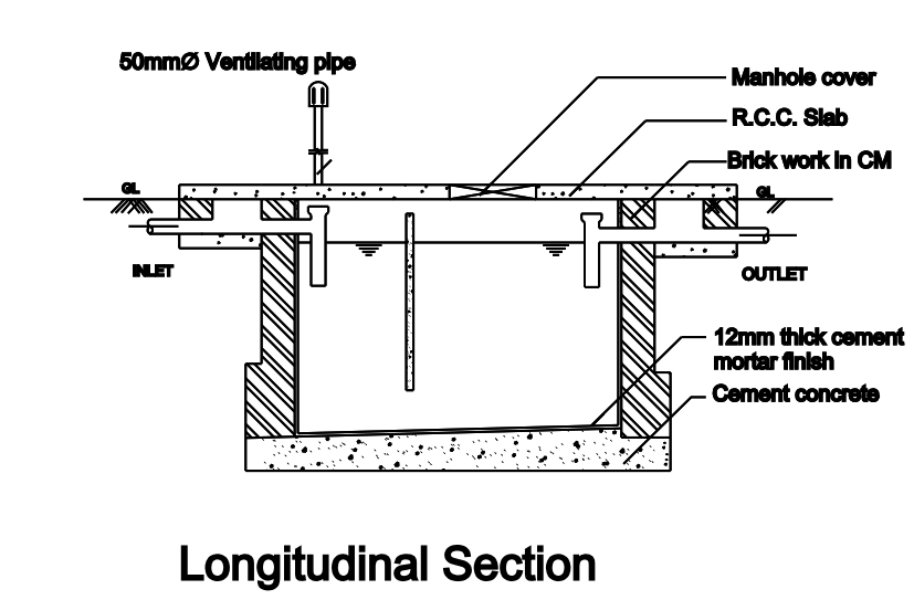
Longitudinal Section (SEPTIC TANK)
