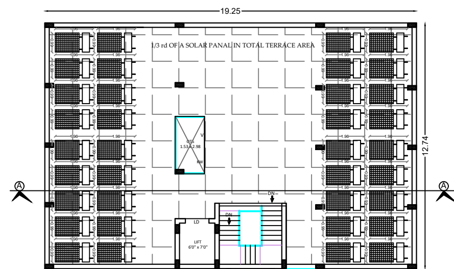
TERREACE FLOOR PLAN
