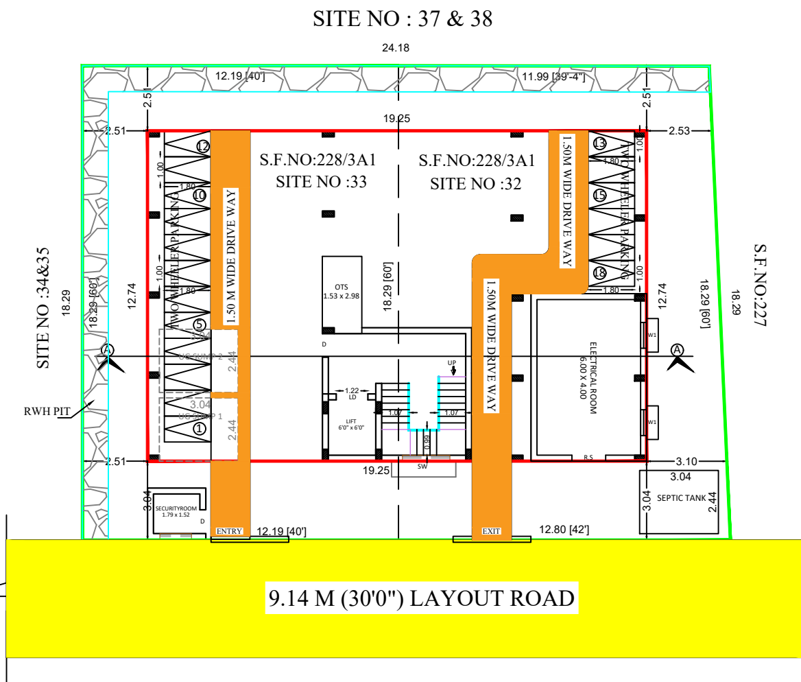
SITE PLAN CUM STILT FLOOR PLAN
