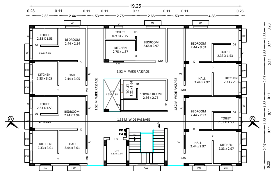
TYPICAL FIRST,SECOND,THIRD,FOURTH FLOOR PLAN
