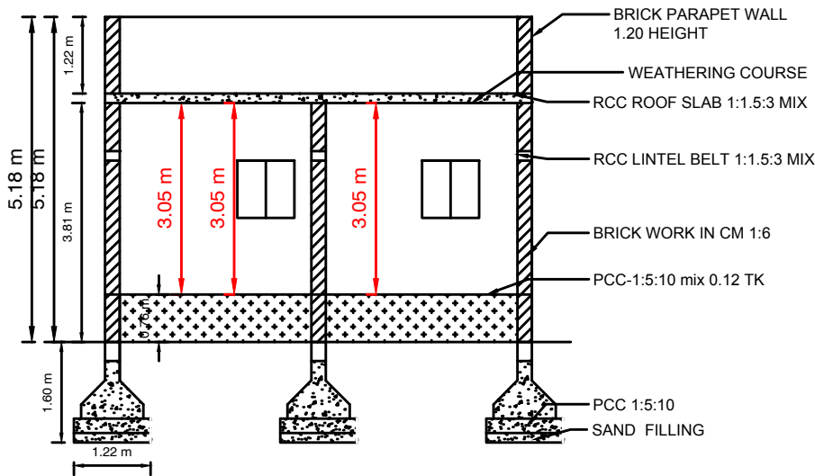
SECTION " AB "
