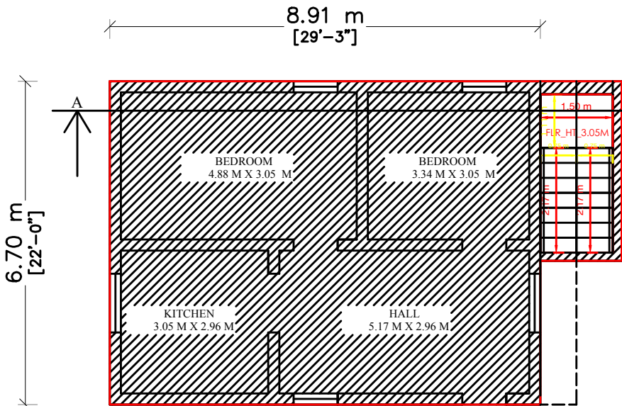
GROUND FLOOR PLAN ( EXISTING )
