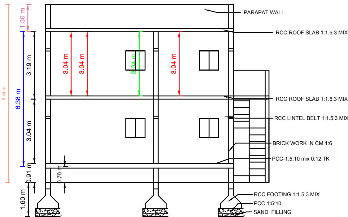
SECTION "AB"
