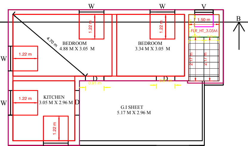
FIRST FLOOR PLAN ( PROPOSED )
