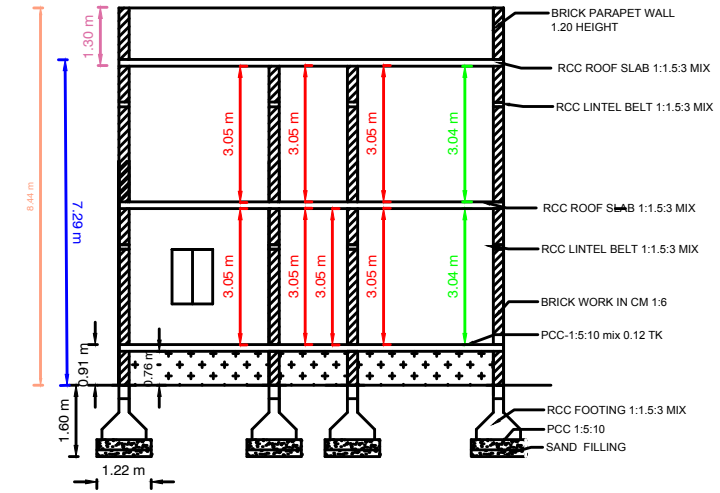
SECTION "AB"
